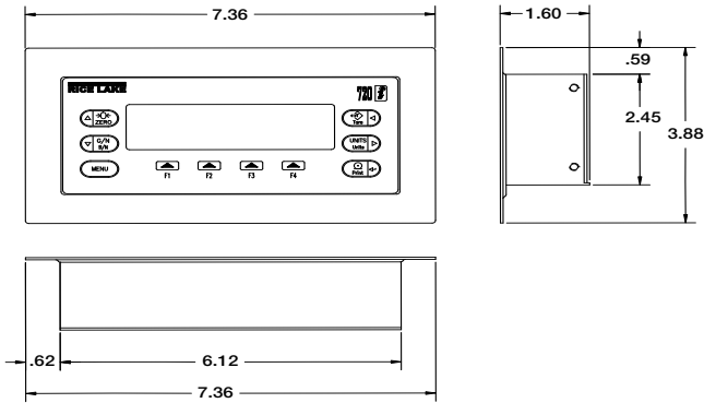
720i Panel Mount
