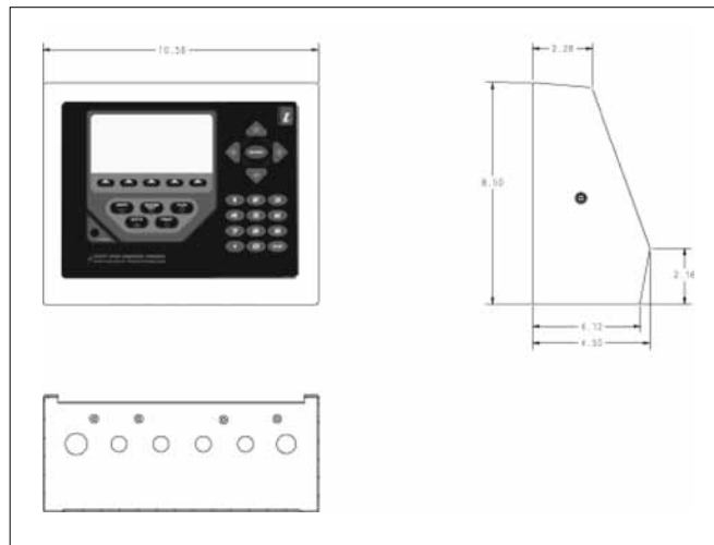
820i Universal Mount
