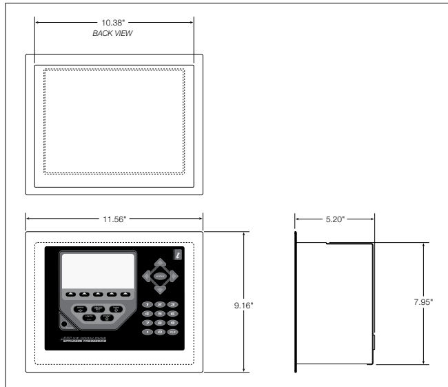
820i Panel Mount
