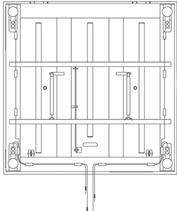
Underdeck View
